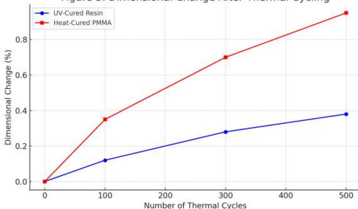
Figure 3. Dimensional Change After Thermal Cycling
